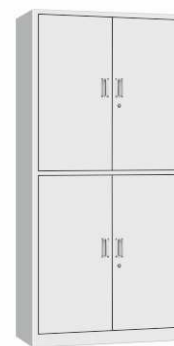
BS-FC-08 H1850*W900*D400mm
